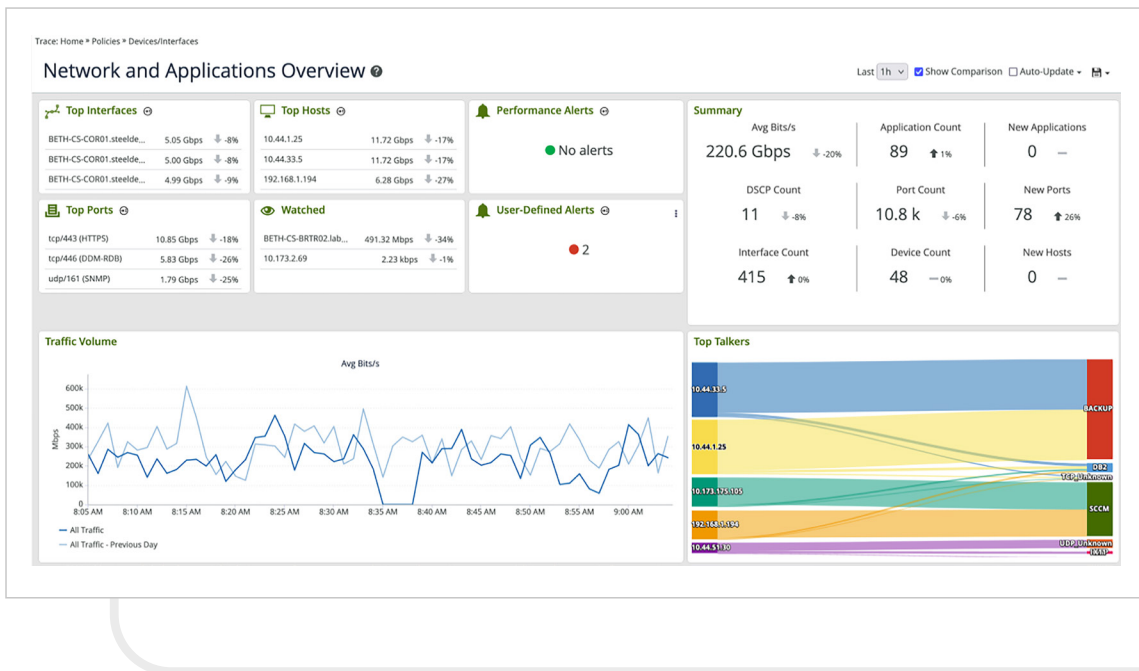
Figure 1: The NetProfiler Home Screen gives each user a personalized summary of network changes, recent alerts, traffic trends, Top Talkers Sankey, and prioritized watch list items.
